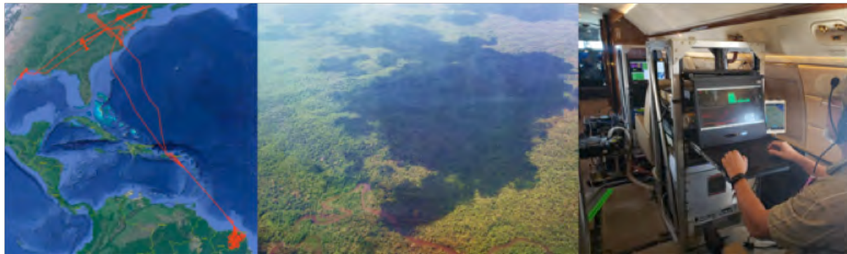
Figure 35. Left: LVIS/GEDI mission flight tracks flown during the deployment. Center: Oblique view of the dense Guiana Shield forest. Photo Credit: David Rabine Right: LVIS instrument and operator inside the GV. Photo Credit: Rob Switzer
