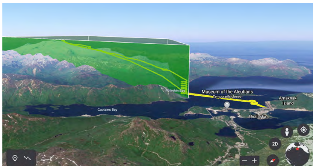
Figure 59. A 3D map showing the flight track of the S2 UAS during a joint USGS/NASA science flight over Makushin Volcano, with the Temporary Flight Restriction indicated in green.
