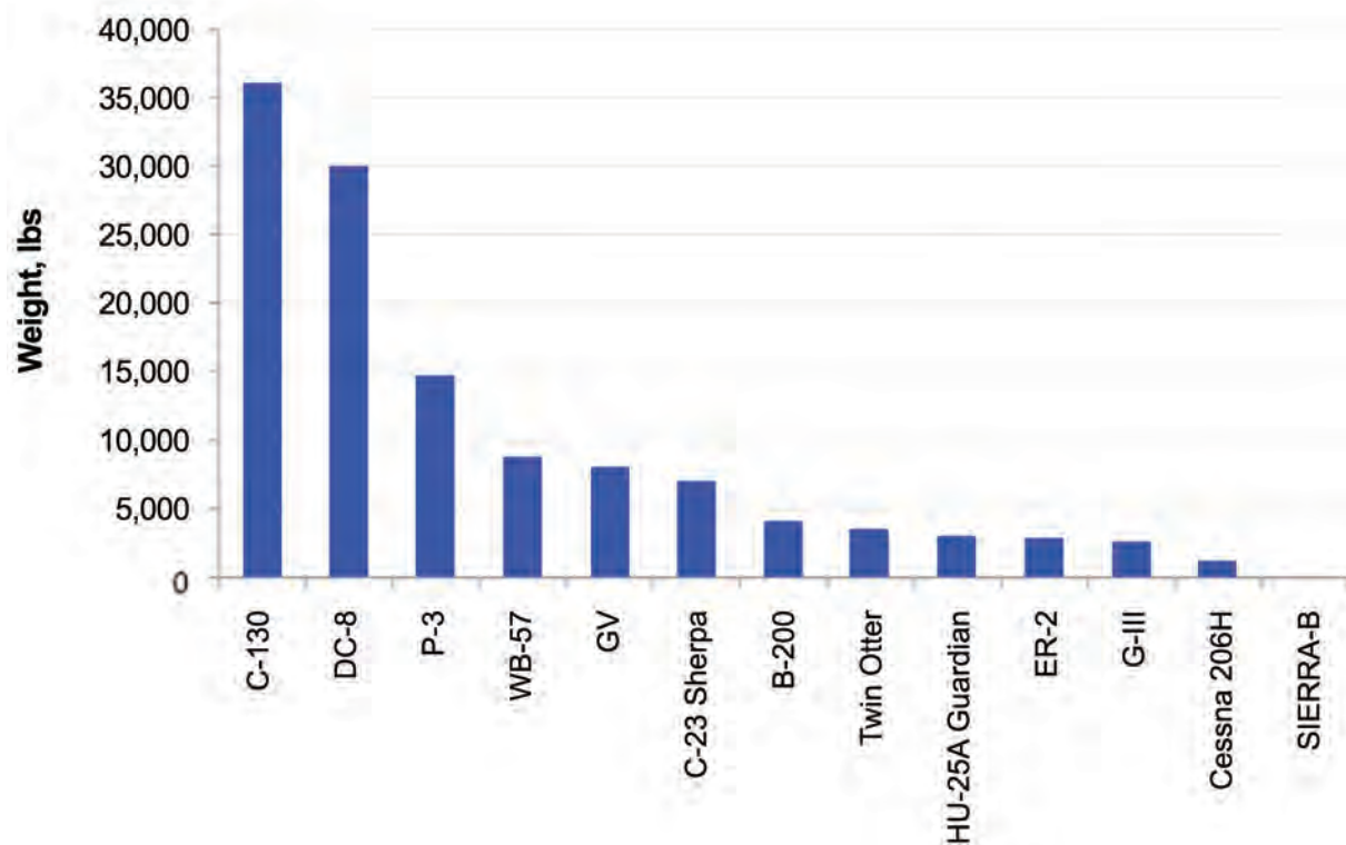
Figure 45. Useful payload weight of NASA aircraft (SIERRA payload weight is approximately 110 lbs.)
