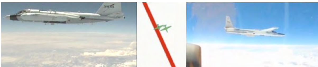
Figure 30. Intercomparison flight of WB-57 (left) and ER-2 (right) at 55,000 ft during overlap of DCOTSS mission and ACCLIP test flights. Insert (middle) shows the aircraft in formation during the flight.
