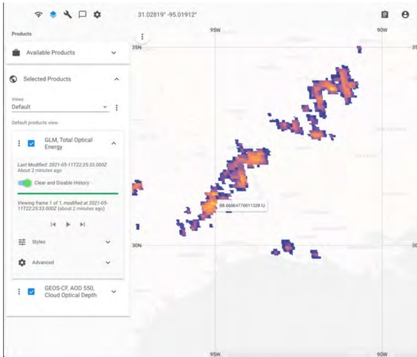
Figure 64. Screenshot showing GLM real time lightning data. The new tool assists mission coordinators with making rapid adjustments when planning science flight segments involving multiple airborne platforms.
