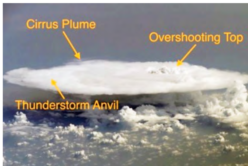
Figure 12. View of an overshooting convective storm, as seen from the International Space Station.
