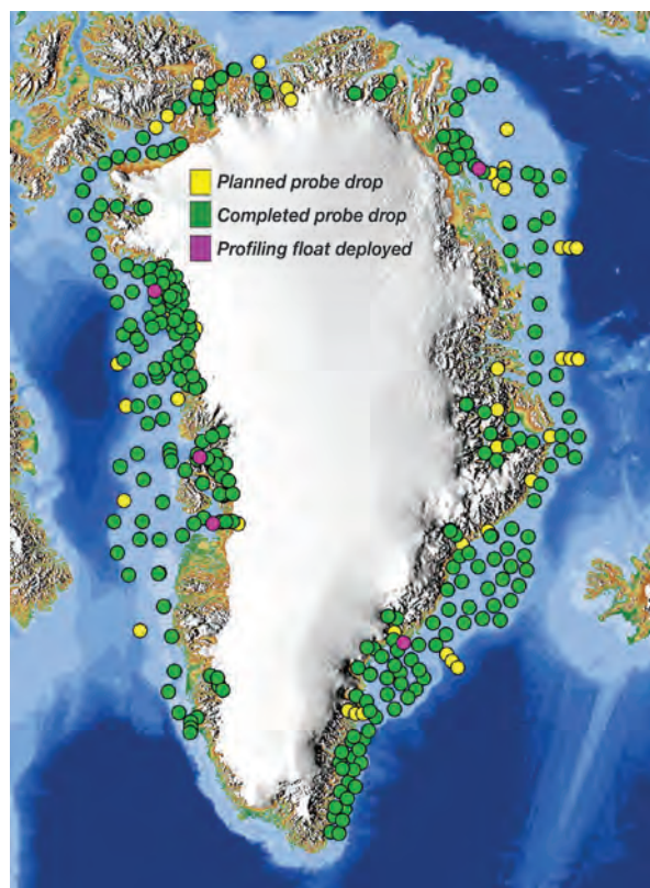
Figure 8. 2021 AXCTD survey of the oceans around Greenland.
