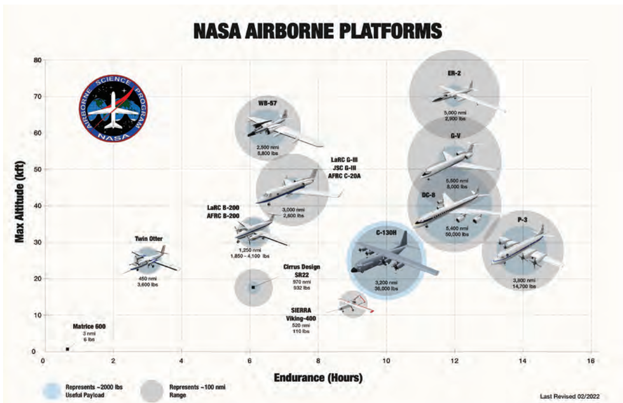
Figure 44. Aircraft capabilities in Altitude, Endurance, Range and Payload.
