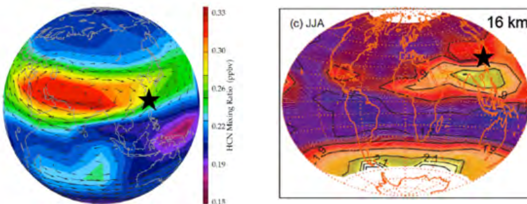
Figure 38. Asian monsoon models. Left: Hydrogen Cyanide measurements at an altitude of 16.5 km. Right: SAGE II data indicating aerosol extinction at an altitude of 16 km.
