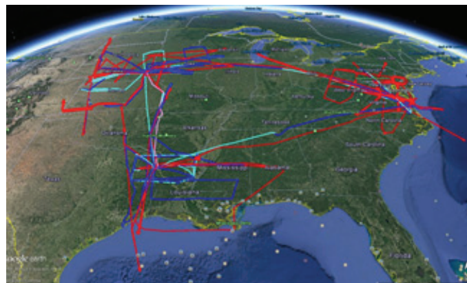
Tracks of the B200 and C130 over the three ACT-America regions (Mid-Atlantic, Mid-West, and South) collecting high-resolution measurements during the Winter-2017 field campaign.
